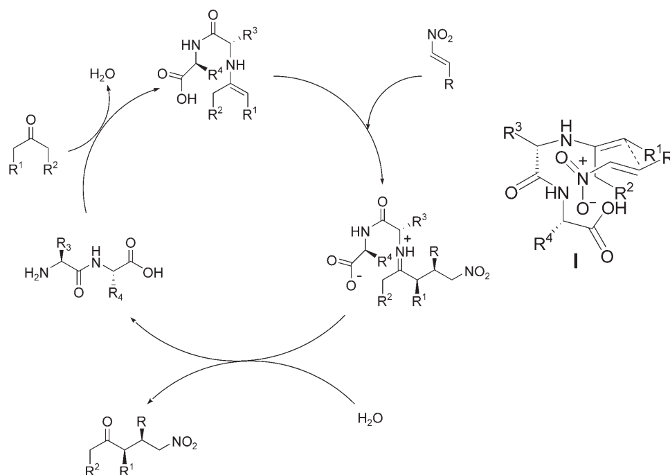
Figure 1. Plausible reaction mechanism and transition state I for the dipeptide-catalyzed asymmetric nitro-Michael reaction.
